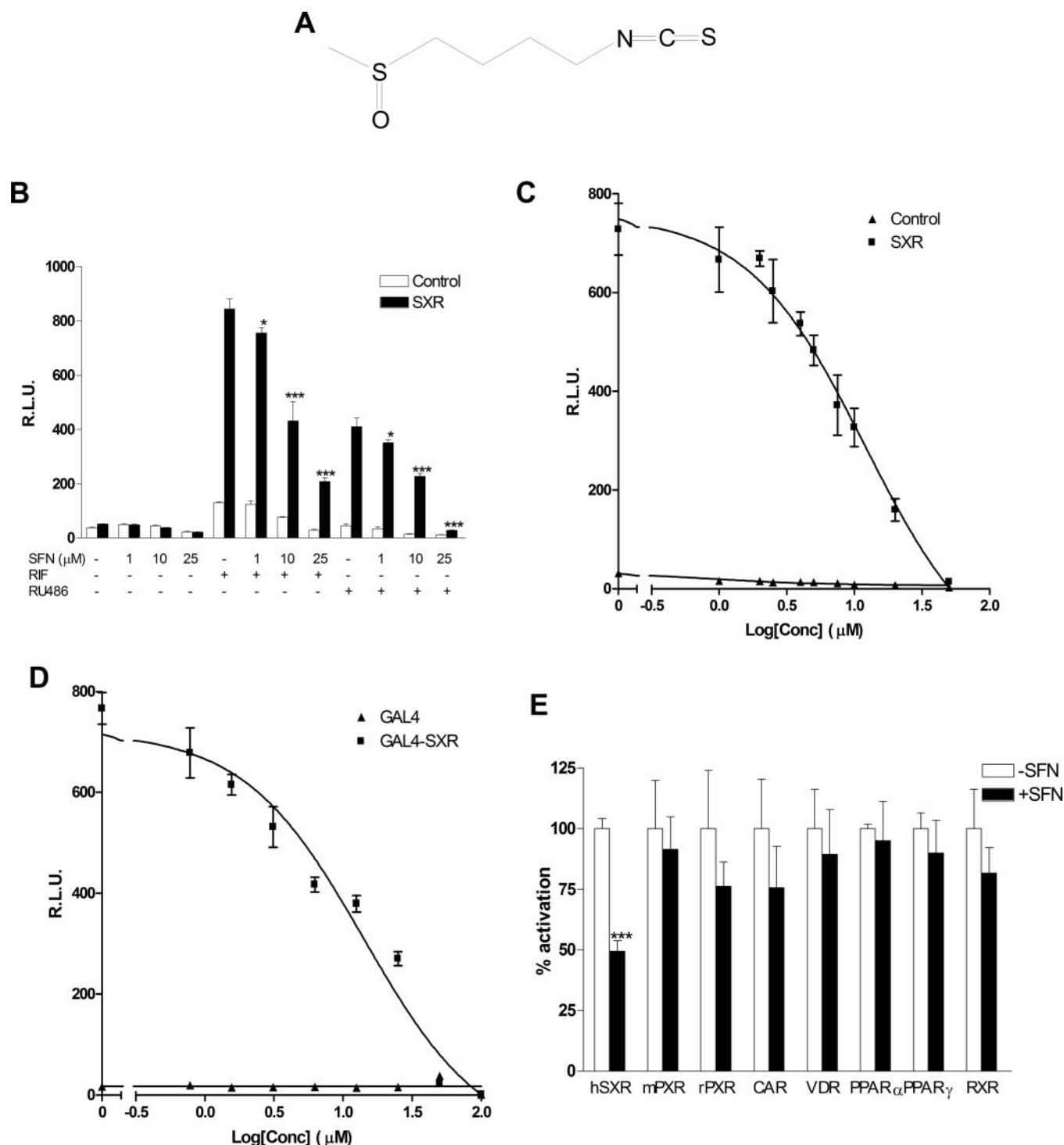
Fig. 1. SFN efficiently inhibits SXR activity. A, structure of SFN (4-methylsulfinylbutyl isothiocyanate). B, HepG2 cells were transiently transfected with full-length SXR together with a CYP3A4-luciferase reporter and CMX- \beta -galactosidase transfection control plasmid. After transfection, cells were treated with control medium or medium containing 10 \mu M RIF or 10 \mu M RU486 in the absence or presence of SFN at the indicated concentrations for 24 h. Results were presented as relative luciferase units (RLUs) normalized to the \beta -galactosidase internal control. C, HepG2 cells were transiently transfected as described above. Cells were treated with 10 \mu M RIF with indicated concentrations of SFN for 24 h. D, HepG2 cells were transiently transfected with GAL4-SXR, a GAL4 reporter fused to luciferase and CMX- \beta -galactosidase transfection control plasmid. Cells were then treated with 10 \mu M RIF and SFN at the indicated concentrations for 24 h. E, HepG2 cells were cotransfected with GAL4 reporter and a series of GAL4 constructs in which the GAL4 DNA binding domain is linked to the indicated nuclear hormone receptor ligand binding domain. Cells were treated with the appropriated ligand or ligand plus 10 \mu M SFN. The ligands used were mouse PXR (mPXR) (10 \mu M PCN), rat PXR (rPXR) (10 \mu M PCN), vitamin D receptor (VDR) [10 nM 1,25(OH) _2 D _3 ], and constitutive androstane receptor (CAR) [1 \mu M 6-(4-chlorophenyl)imidazo[2,1- b ]-[1,3]thiazole-5-carbaldehyde O -(3,4-dichlorobenzyl)oxime], PPAR \alpha (10 \mu M Wy-14,643), PPAR \gamma (10 \mu M troglitazone), and retinoid X receptor (RXR) (100 nM 9- cis -retinoic acid). Results in the presence of SFN are presented as percentage of activation relative to the normalized luciferase values in the presence of ligands (100%). Statistically significant expression compared with control group (-SFN), respectively, is marked with asterisks: *, P < 0.05 ; **, P < 0.01 ; and ***, P < 0.001 ( n = 3 ; Student's t test).
